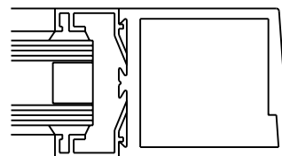
DOUBLE GLAZED OPTION
