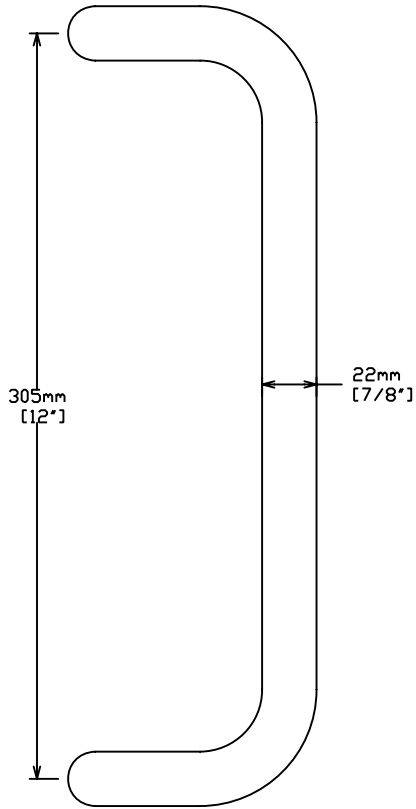
1 Side Mount
